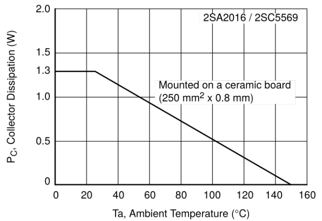
Figure 19. P_C - T_a
