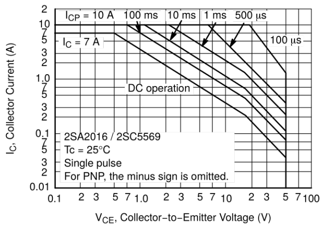
Figure 18. ASO
