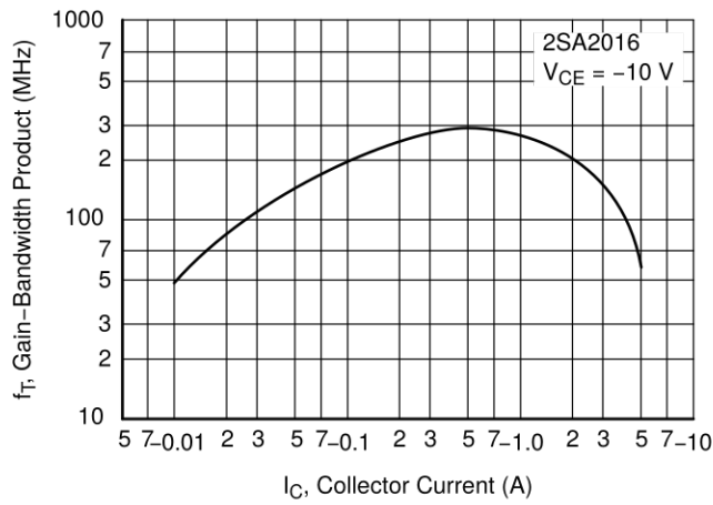
Figure 16. f_T - I_C
