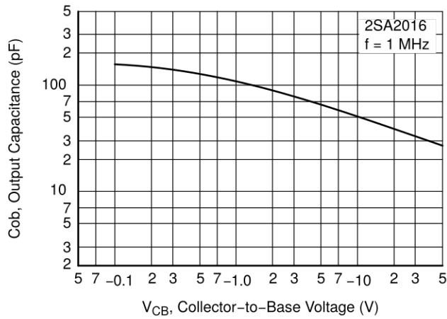
Figure 14. Cob - V_{CB}
