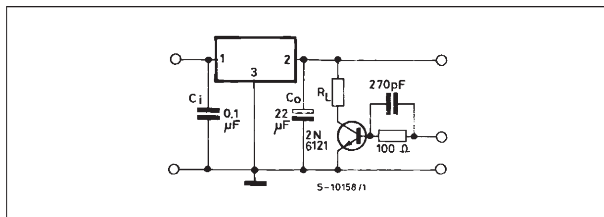
Figure 2 : Load Rejection.
