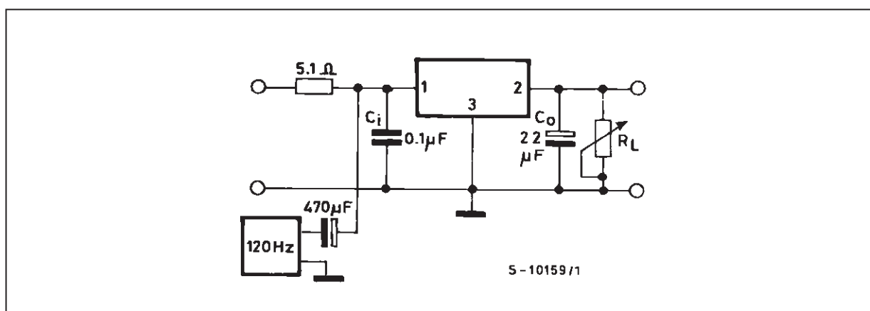
Figure 3 : Ripple Rejection.
