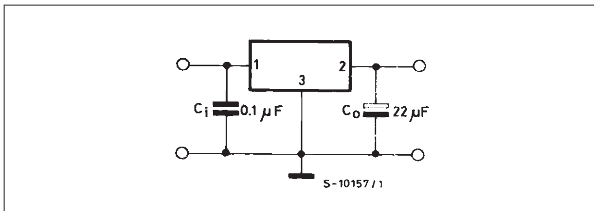
Figure 1 : DC Parameter.
