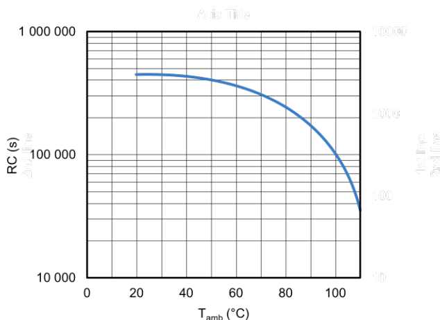
Insulation resistance as a function of ambient temperature
